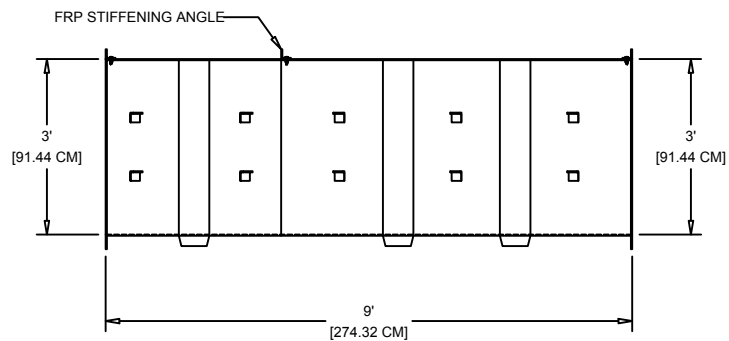
ELEVATION VIEW
