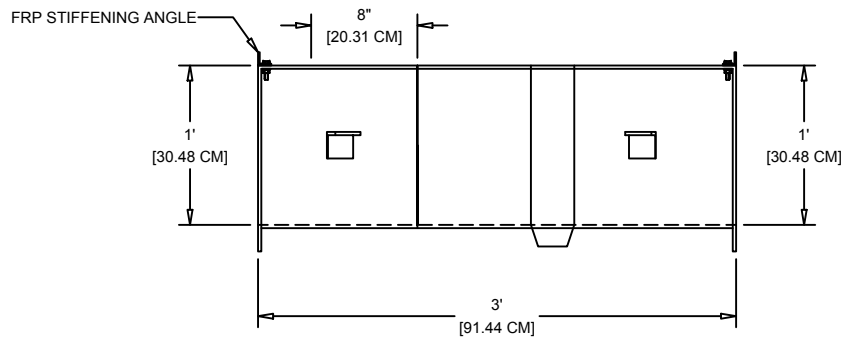
ELEVATION VIEW
